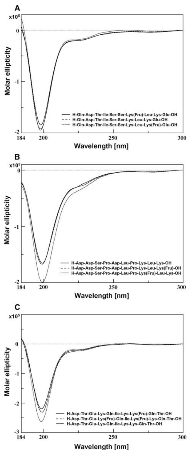
Fig. 2 CD spectra of the glycated albumin fragments: A: peptides derived from the sequence H-Gln-Asp-Thr-Ile-Ser-Ser-Lys-Leu-Lys-Glu-OH, B: peptides derived from the sequence H-Asp-Asp-Ser-Pro-Asp-Leu-Pro-Lys-Leu-Lys-OH and C: peptides derived from the sequence H-Asp-Thr-Glu-Lys-Gln-Ile-Lys-Lys-Gln-Thr-OH. All spectra were measured in water at pH 7, details are given in “Materials and methods”
