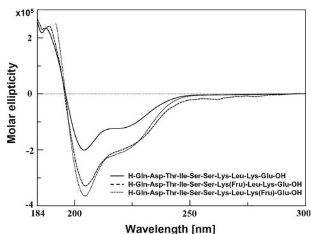
Fig. 3 CD spectra of the glycated peptides: H-Gln-Asp-Thr-Ile-Ser-Ser-Lys-Leu-Lys-Glu-OH, H-Gln-Asp-Thr-Ile-Ser-Ser-Lys-Leu-Lys(Fru)-Glu-OH and H-Gln-Asp-Thr-Ile-Ser-Ser-Lys(Fru)-Leu-Lys-Glu-OH. Spectra were measured in TFE, details are given in “Materials and methods”
